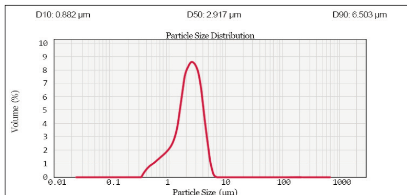
Ceroxid HD R2536 PSD laser particle size distribution analyzer
